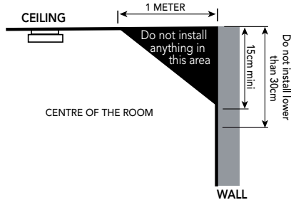
FIG.3 Detector position
